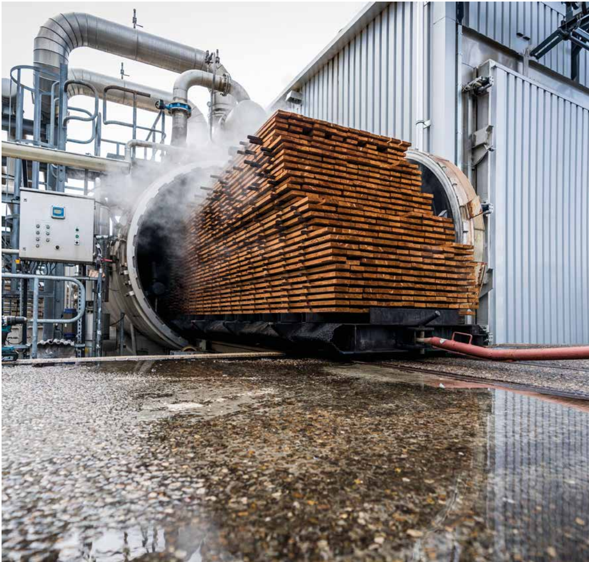
Steaming (hydrothermolysis)
